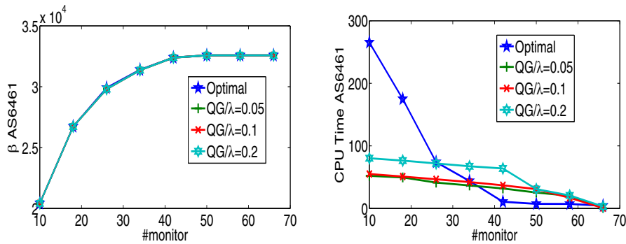
Fig. 5. MMRP performance for quasi-greedy algorithm for AS6461.
