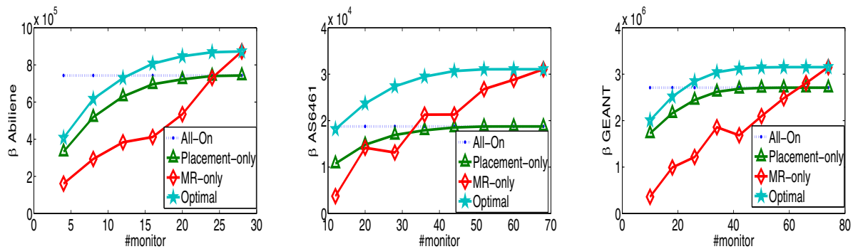
Fig. 2. Compare optimal MMPR with default cases for Abilene, AS6461 and GEANT.
